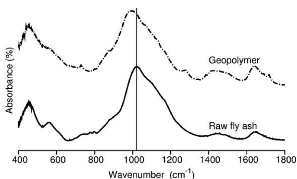
Fig. 14. FTIR spectra of RFA and geopolymer paste.
