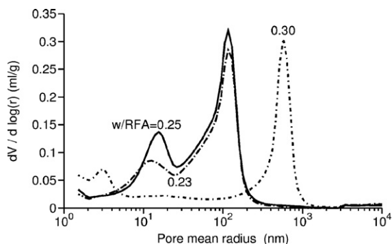
Fig. 13. MIP pore-size distribution in geopolymer pastes with three water/RFA mass ratios.
