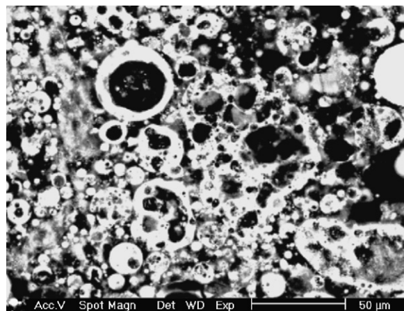
Fig. 11. Polished section of geopolymer paste (BSE).
